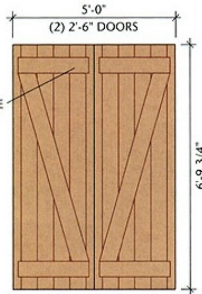
INSIDE ELEVATION
