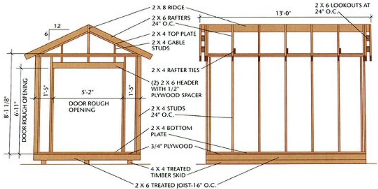
FRONT FRAMING ELEVATION
