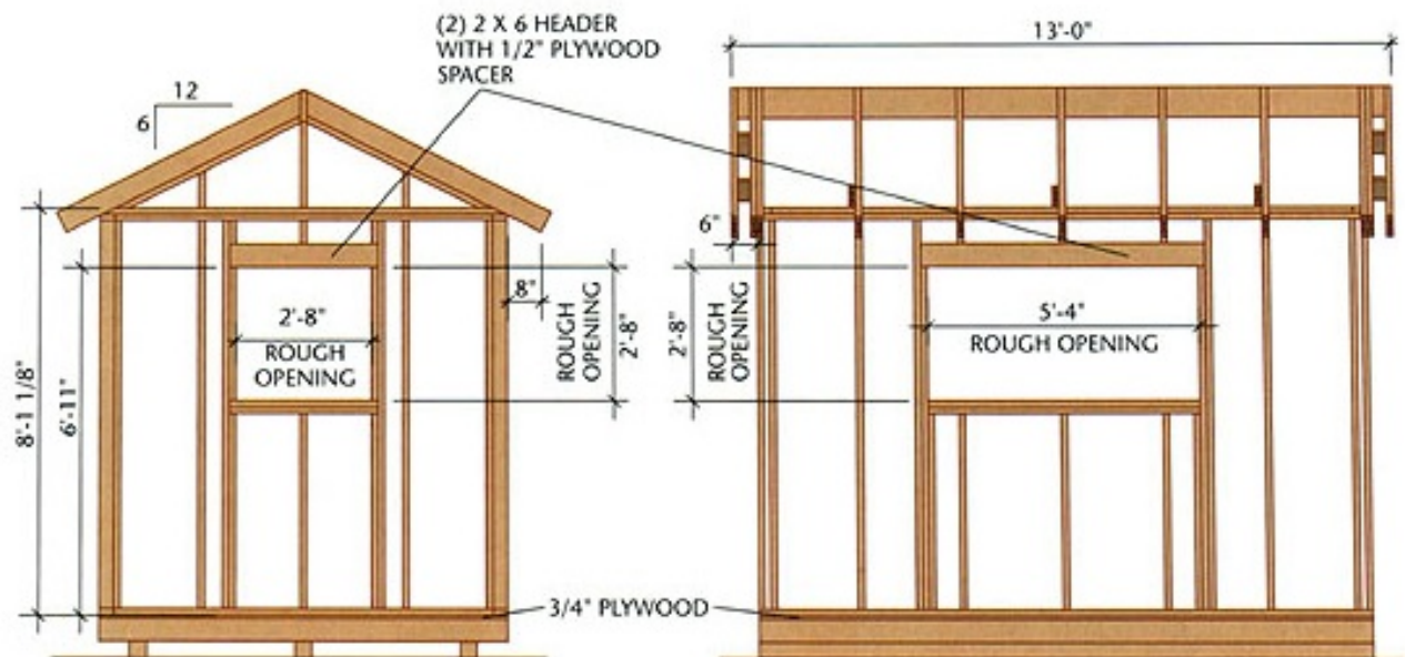
REAR FRAMING ELEVATION
